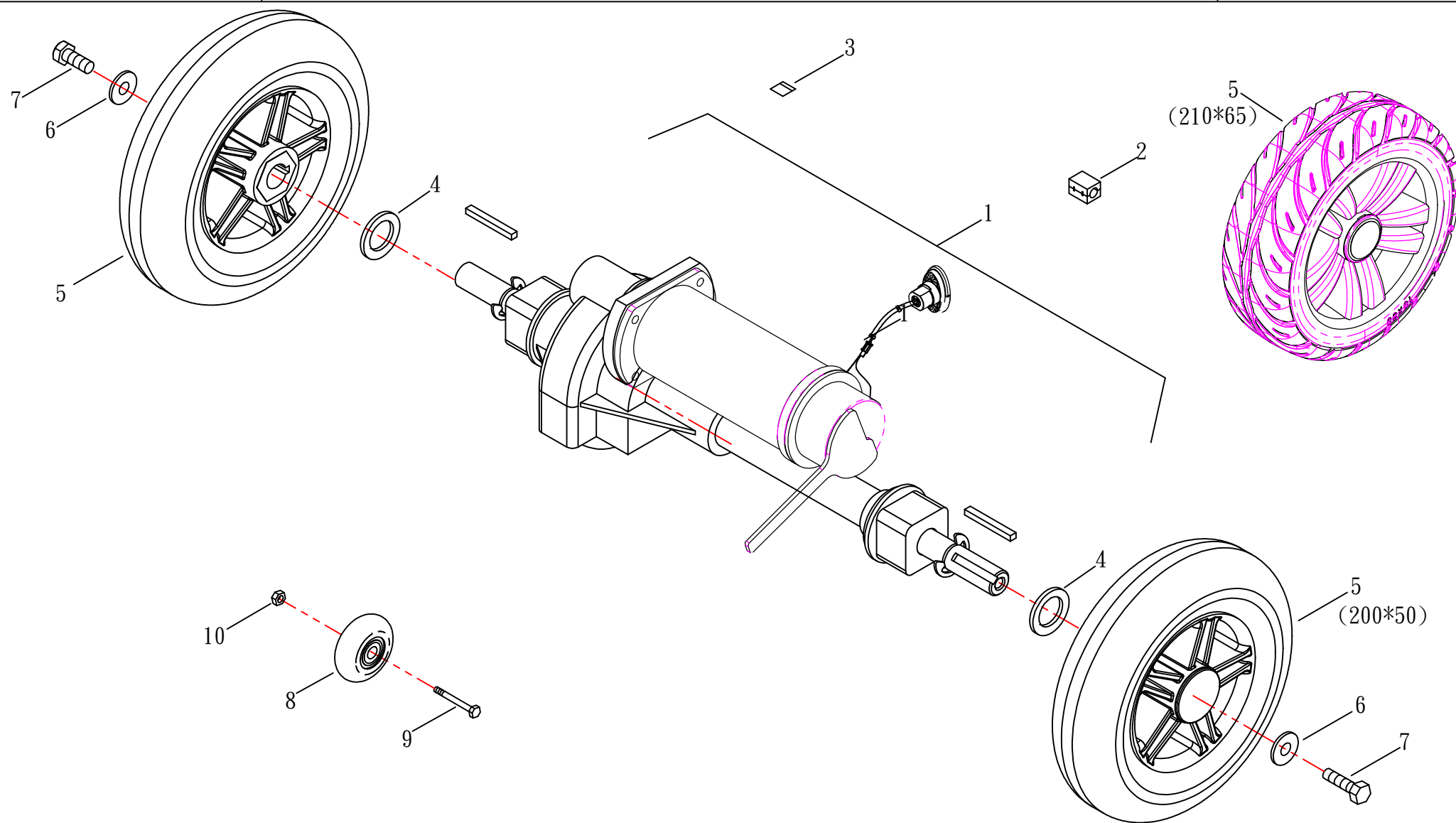
(FIG. 6) REAR WHEEL & MOTOR ASSEMBLY
