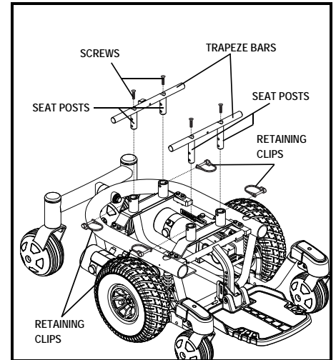
Figure 16. Seat Height Adjustment - Trapeze Bars
