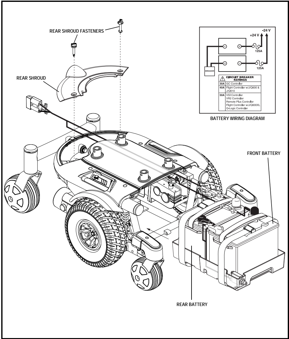
Figure 28. Battery Installation
