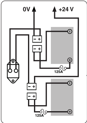
Battery Wiring Diagram Label
